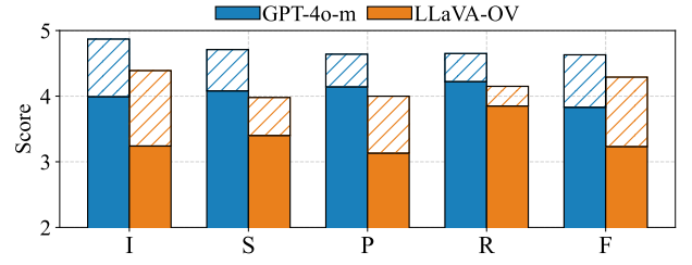
Figure 6: Comparison of explanation quality with and without R³CoT on the FakeTT dataset. I: Informativeness, S: Soundness, P: Persuasiveness, R: Readability, F: Fluency.
