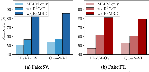
Figure 4: Generalizability analysis on adding our R³CoT and SLReviewer to base MLLM.
