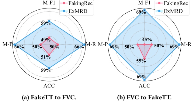
Figure 5: Generalizability analysis through cross-dataset experiments on the FakeTT and FVC datasets.
