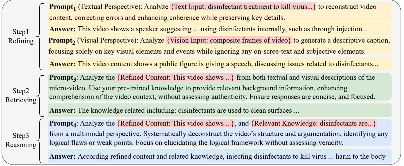
Figure 3: An illustration of three-step prompting of our proposed R 3 CoT. Step 1, prompt MLLM to organize chaotic and misleading video input; Step 2, instruct MLLM to generate rumor-relevant knowledge; Step 3, guide MLLM to conduct inference to cross-verify the refined and retrieved content.
