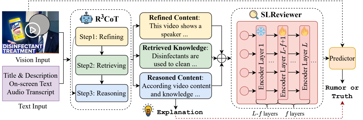
Figure 2: The structure of our proposed ExMRD framework. (1) The R^3CoT process prompts MLLMs to refine the video content, retrieve domain knowledge, and reason to provide explanations. (2) The SLReviewer is to distill the explainable evidence from R^3CoT to facilitate reliable rumor detection.
